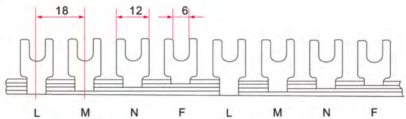
FBB-4P
