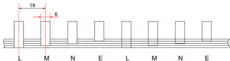
DZ47-4P
